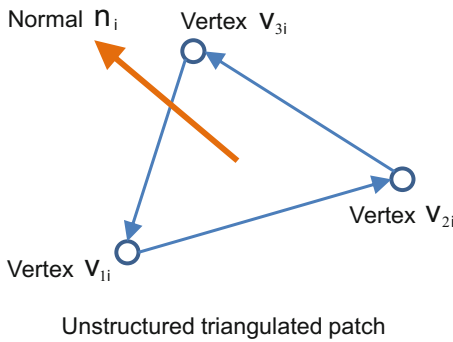
Fig. 3 Unstructured triangulated patch and an example of STL file
