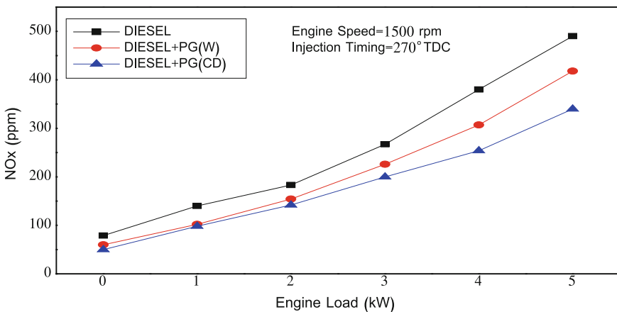
Fig. 17 Effect of brake power on NO x emission at varying load in dual fuel mode
