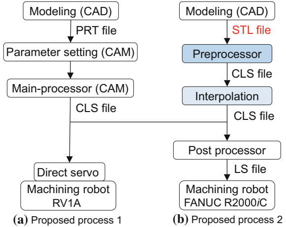
Fig. 1 Comparing the proposed two processes for robotic machining
