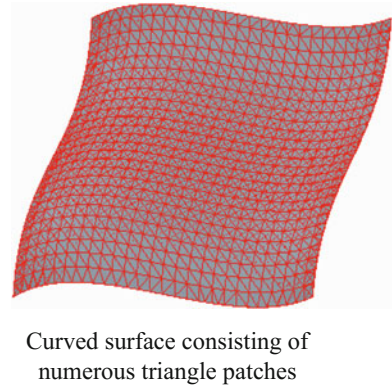
Fig. 3 Unstructured triangulated patch and an example of STL file
