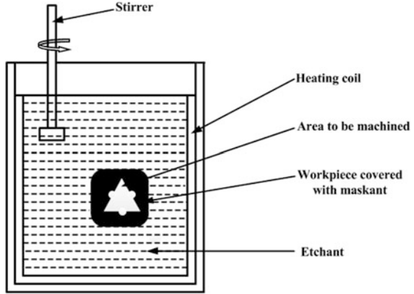
Fig. 18 A schematic diagram of chemical machining process
