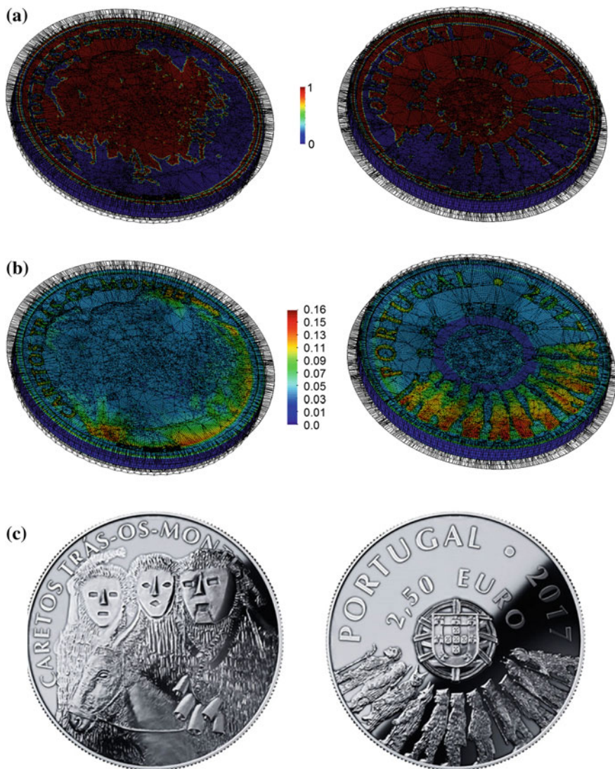
Fig. 12 Finite element estimates of the a contact/no-contact distribution and of b the z -distances (mm) between the surfaces of the disk and the obverse and reverse dies for a die stroke corresponding to point 'P' in Fig. 11. The collection coin dedicated to Portuguese ethnography is shown in (c) for reference purposes
